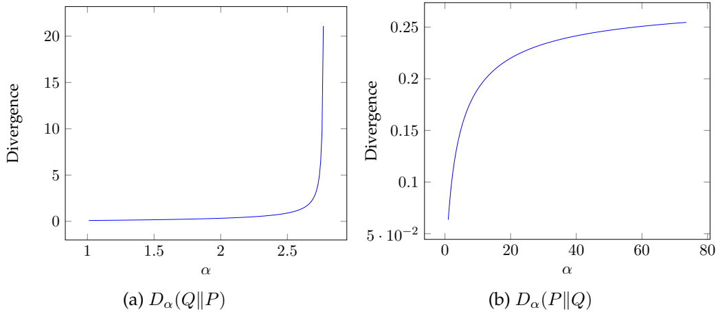
Figure 2.1 – Divergence of two Gaussian functions such that \mu_P = 4, \sigma_P = 4 and \mu_Q = 5, \sigma_Q = 5 .
